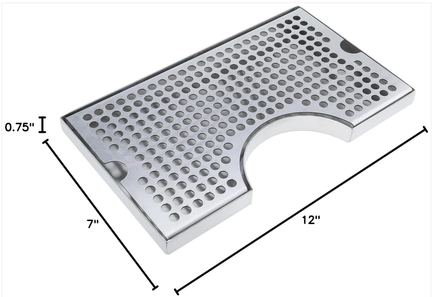
Image: The drip tray with key dimensions (length, width, height) clearly marked, providing a visual reference for its size.
