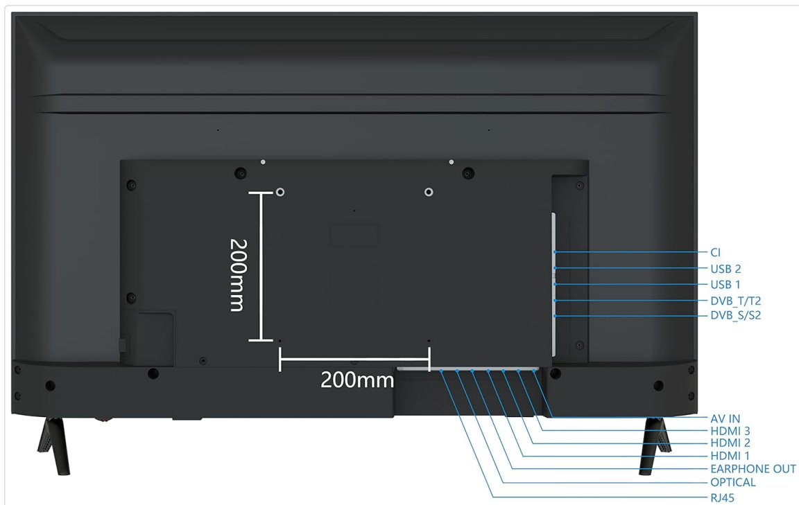
Figure 5.2: Rear view with VESA mounting points and port layout.
