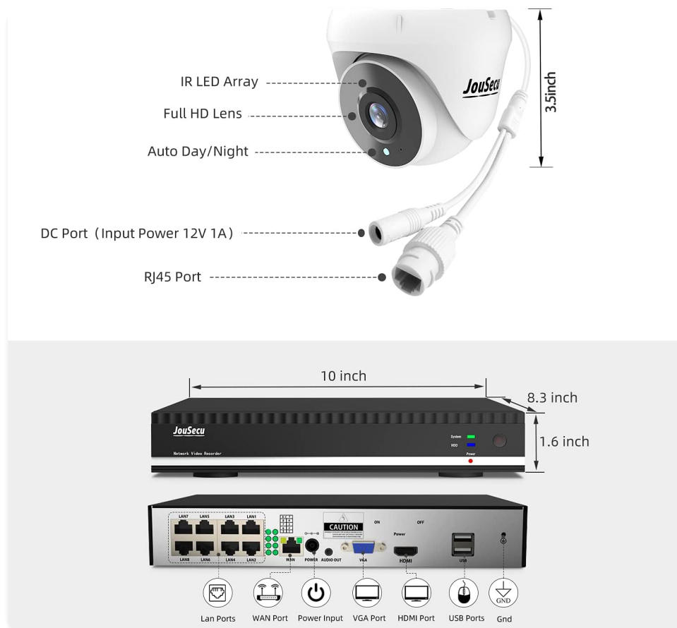
Figure 7.1: NVR and Camera Dimensions & Ports
