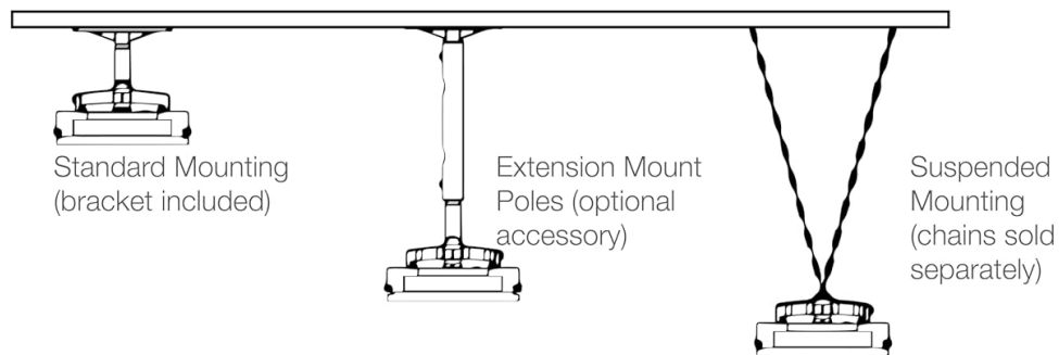
Image 2: Ceiling Mount Options.
