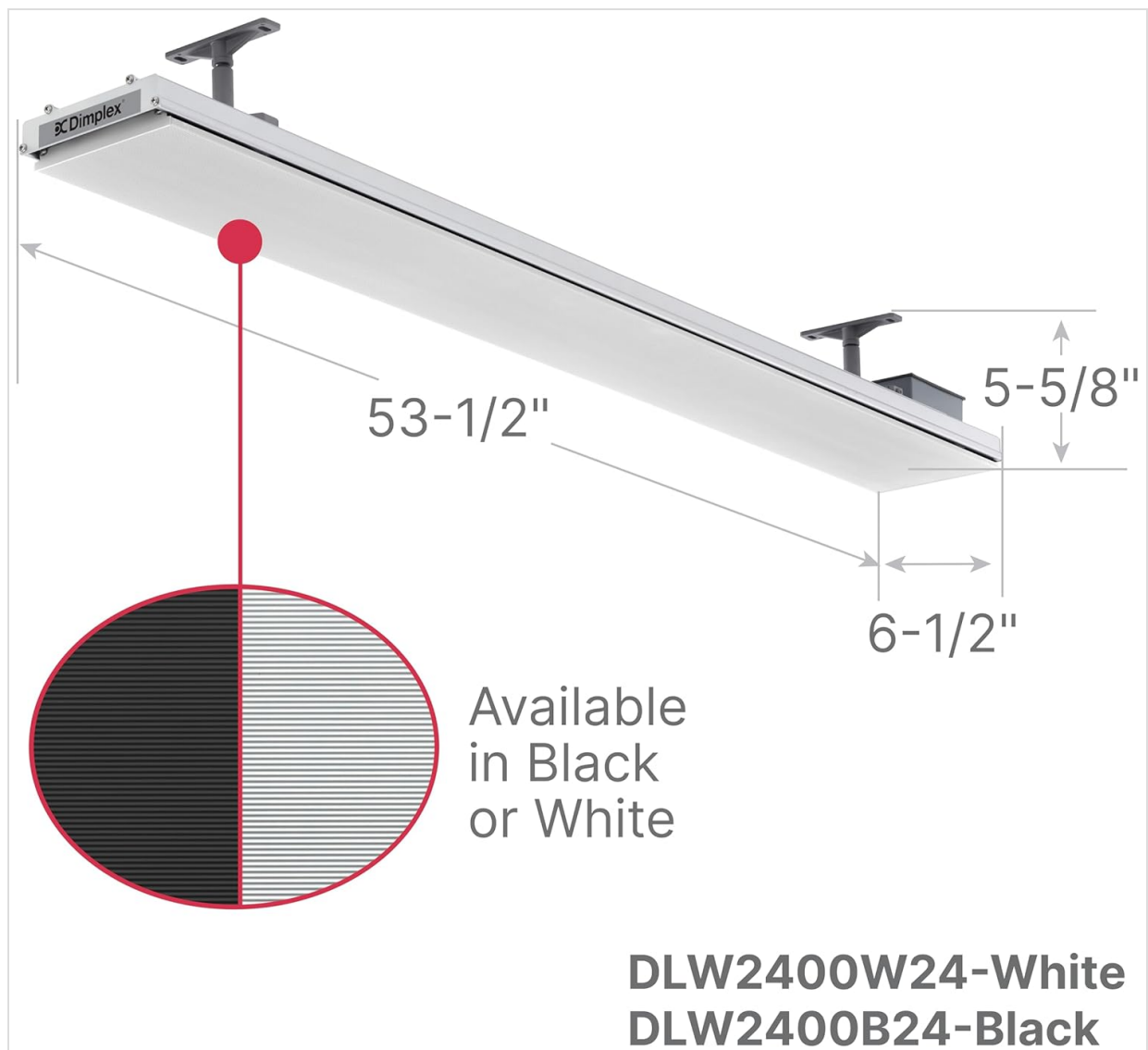
Image 4: Product Dimensions and Color Options.
