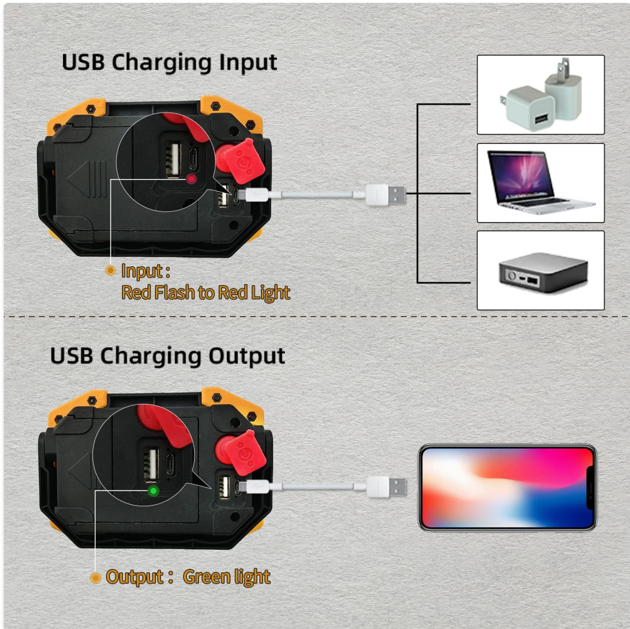
Image 4.1: USB Charging Input and Output ports.
