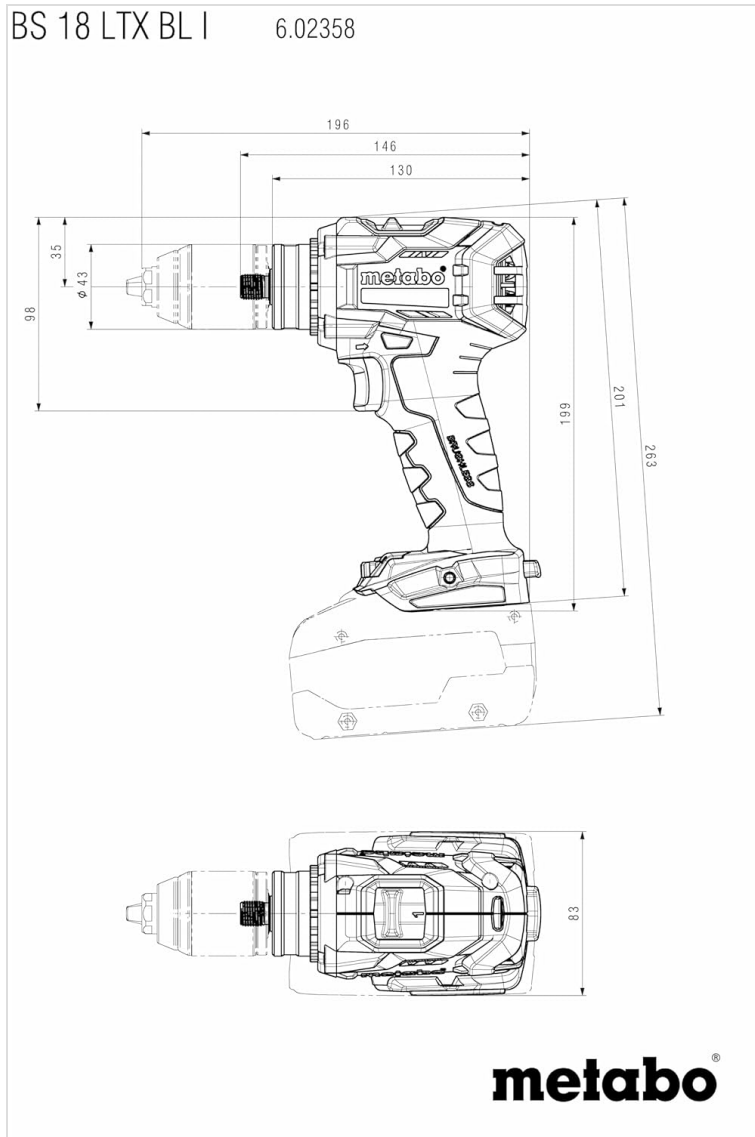
Figure 2: Technical drawing illustrating the dimensions of the Metabo BS 18 LTX BL I drill driver. This diagram provides precise measurements for the tool's length, height, and width, including the chuck diameter (43mm Euro collar).
