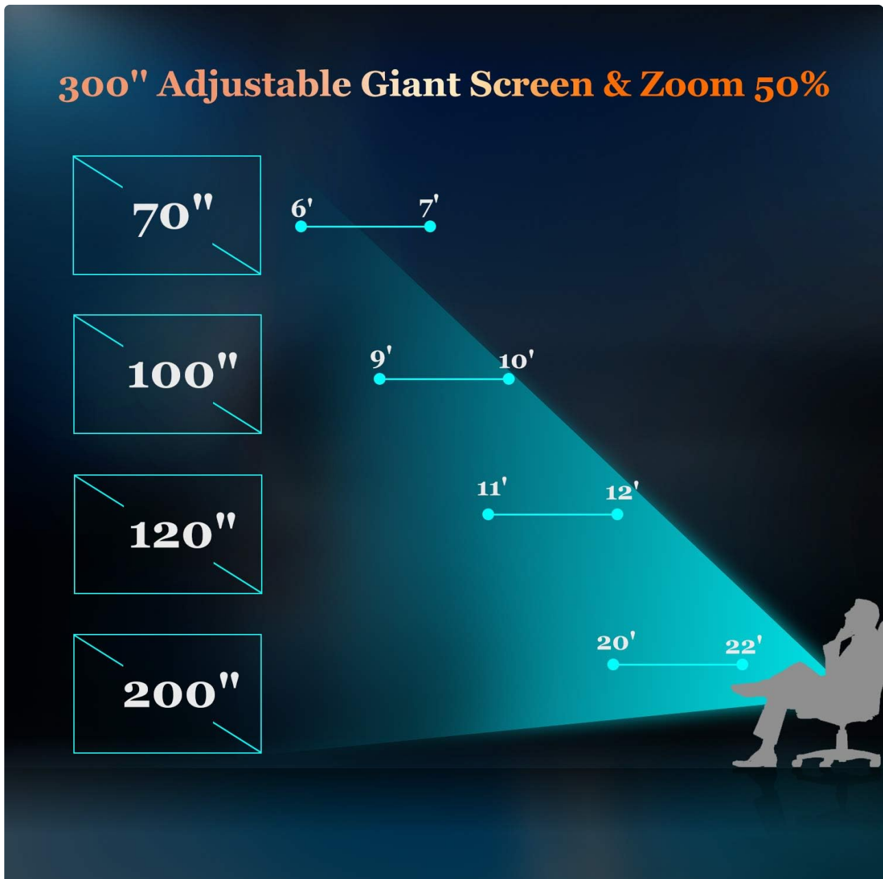
Figure 5: Recommended projection distances for different screen sizes (e.g., 70" at 6-7ft, 100" at 9-10ft, 120" at 11-12ft, 200" at 20-22ft).
