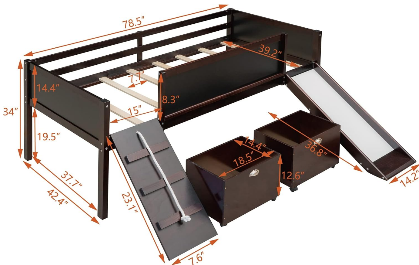
Image: A technical diagram illustrating the precise measurements of the Bellemave Twin Low Loft Bed, including the bed frame, slide, climbing ladder, and storage boxes.
