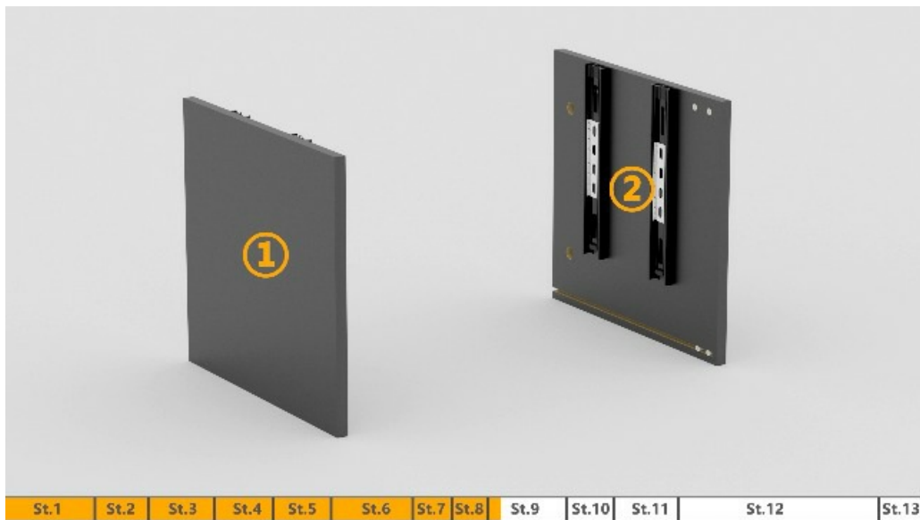
Figure 2: Exploded view of nightstand components
