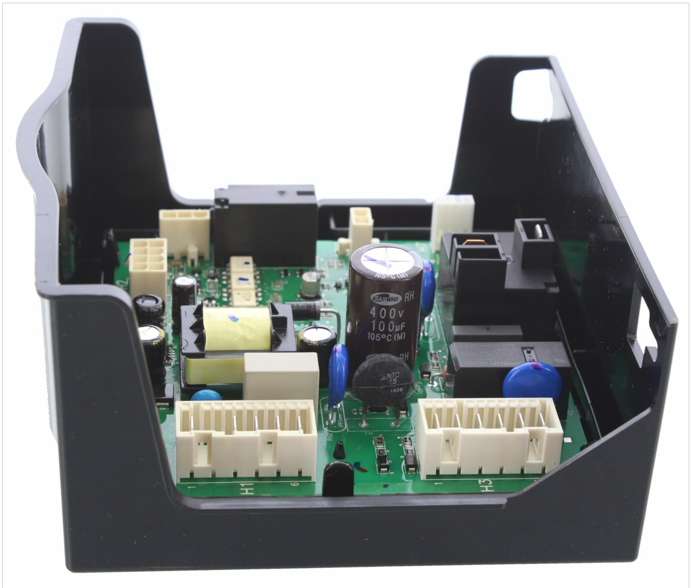
Figure 1: The ALLIANCE LAUNDRY SYSTEMS D513797P Dryer Output Control Board. This image shows the green circuit board housed within a black plastic casing, featuring various electronic components, connectors, and a large capacitor. The board is designed to manage the output functions of a commercial dryer.
