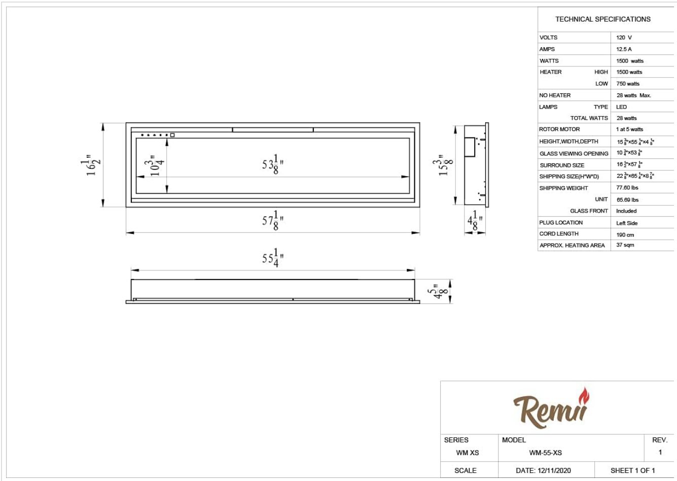
Image 4.1: Technical drawing showing the dimensions and electrical specifications for the WM-55-XS model, useful for installation planning.
