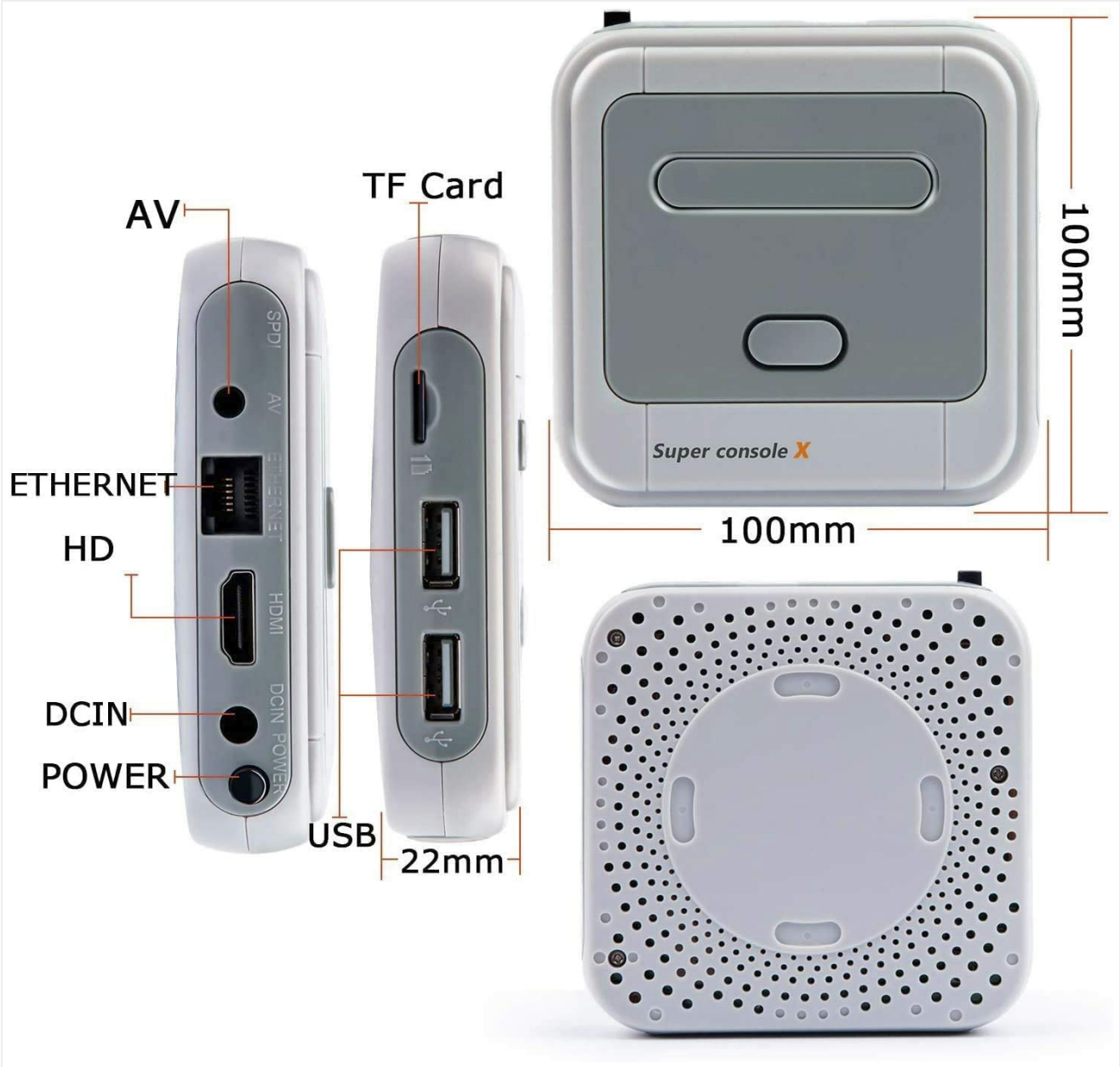
Image 3.1: Super Console X port layout and dimensions.
