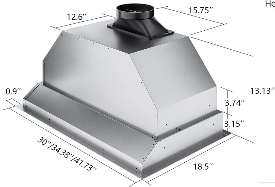
Figure 2: Range Hood Dimensions and Recommended Installation Height.
