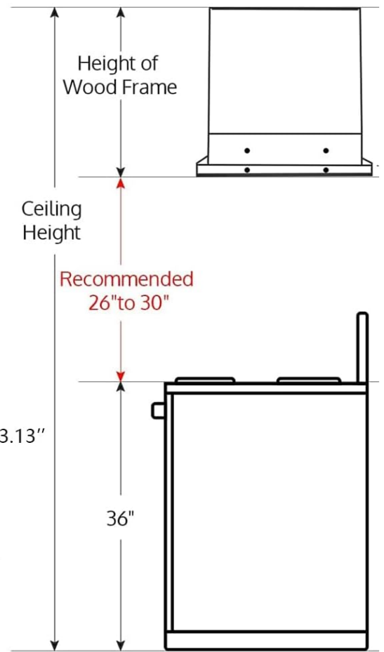
Figure 2: Range Hood Dimensions and Recommended Installation Height.
