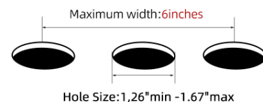
Figure 4: Faucet installation on a 3-hole sink using the deck plate. Maximum width: 6 inches. Hole size: 1.26" - 1.67" minimum to maximum.
