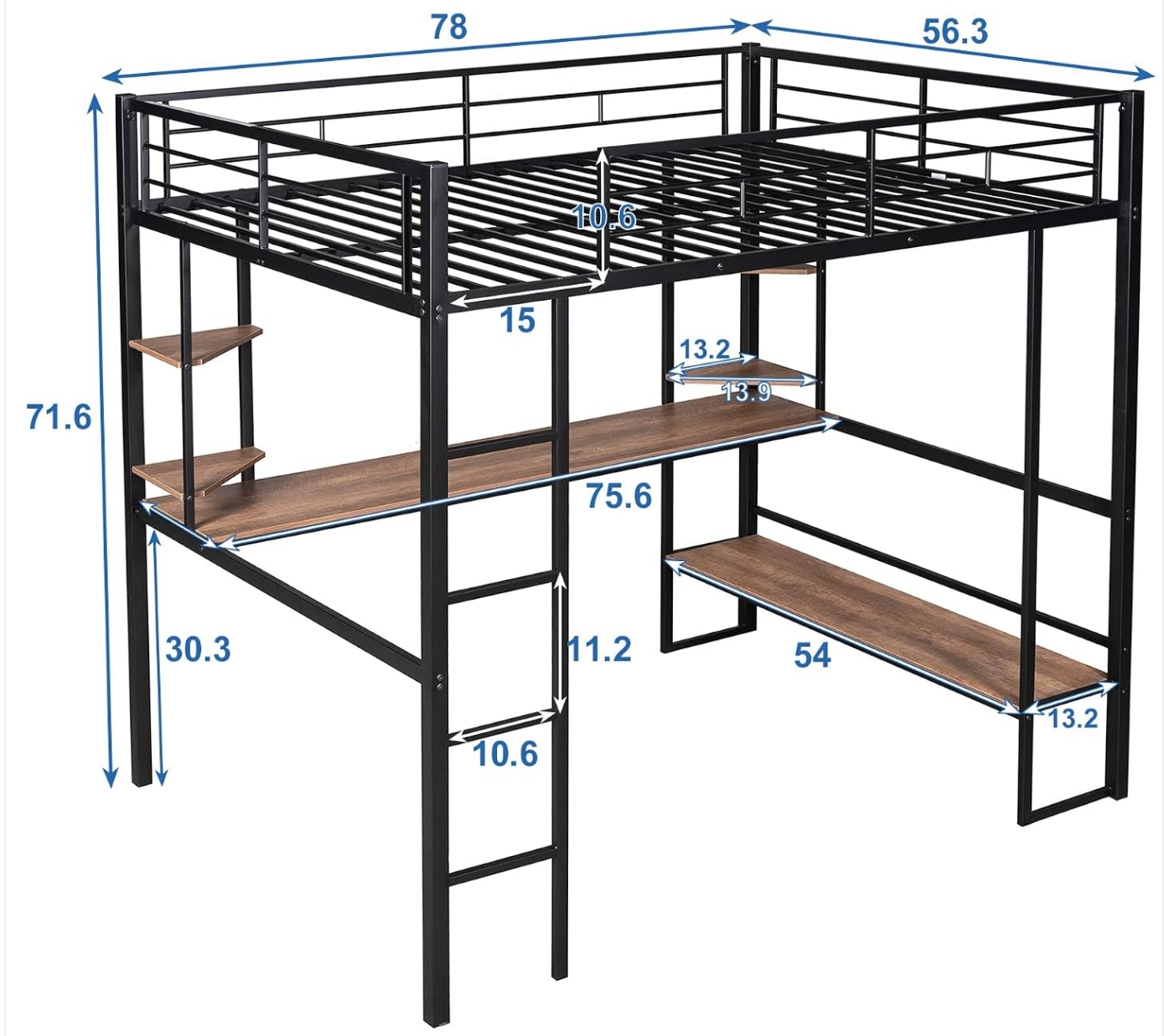
Image: A detailed diagram illustrating the overall dimensions of the loft bed, including length, width, height, and specific measurements for the desk and shelves in inches.
