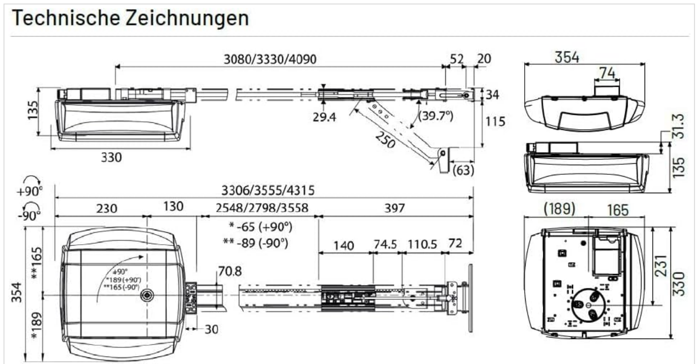
Figure 3.1: Technical dimensions for installation planning.
