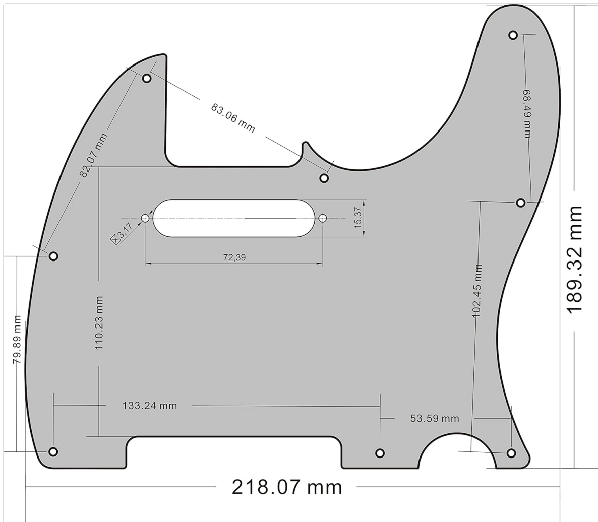
Figure 3: Dimensional drawing of the pickguard, showing key measurements for fitment.
