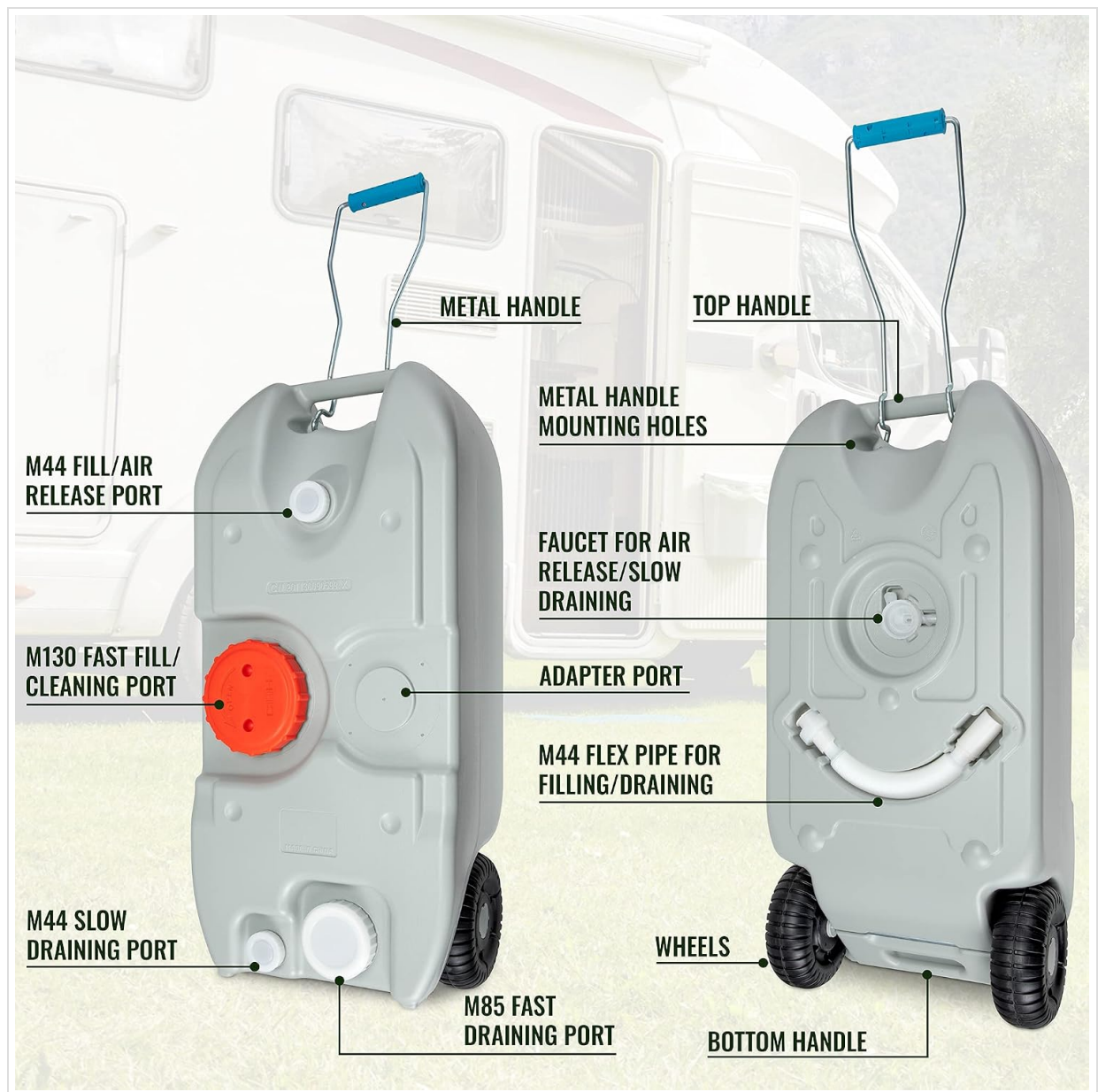
Image: A detailed diagram labeling the various ports, handles, and wheels of the waste holding tank.
