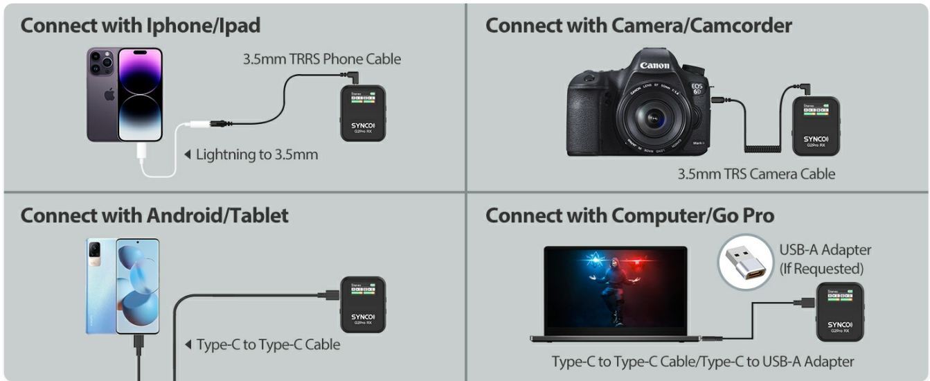
Figure 3: Connection diagrams for smartphones, cameras, and computers.
