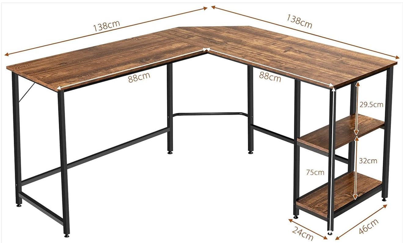
Figure 2: Dimensional diagram of the L-shaped desk, illustrating its length, width, and height for planning your space.
