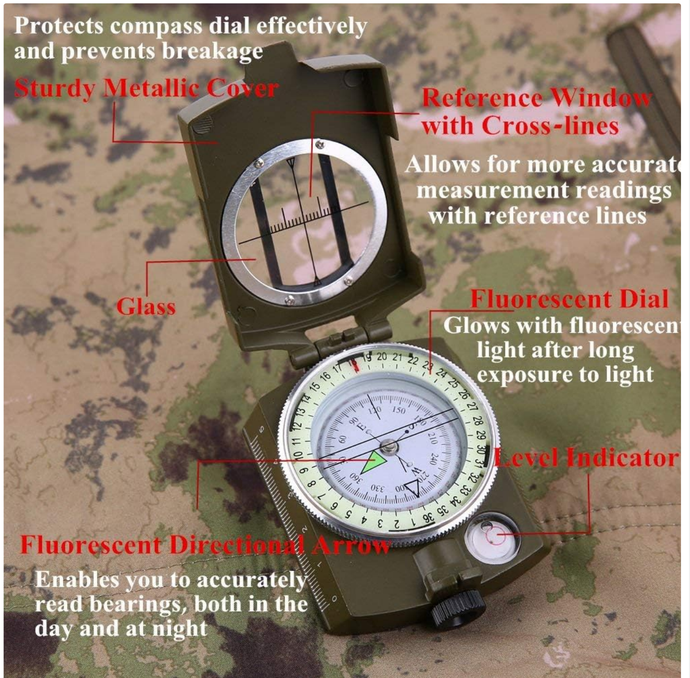
Image: A detailed view of the compass, pointing out key components such as the sturdy metallic cover, reference window with cross-lines, fluorescent dial, level indicator, and fluorescent direction arrow.
