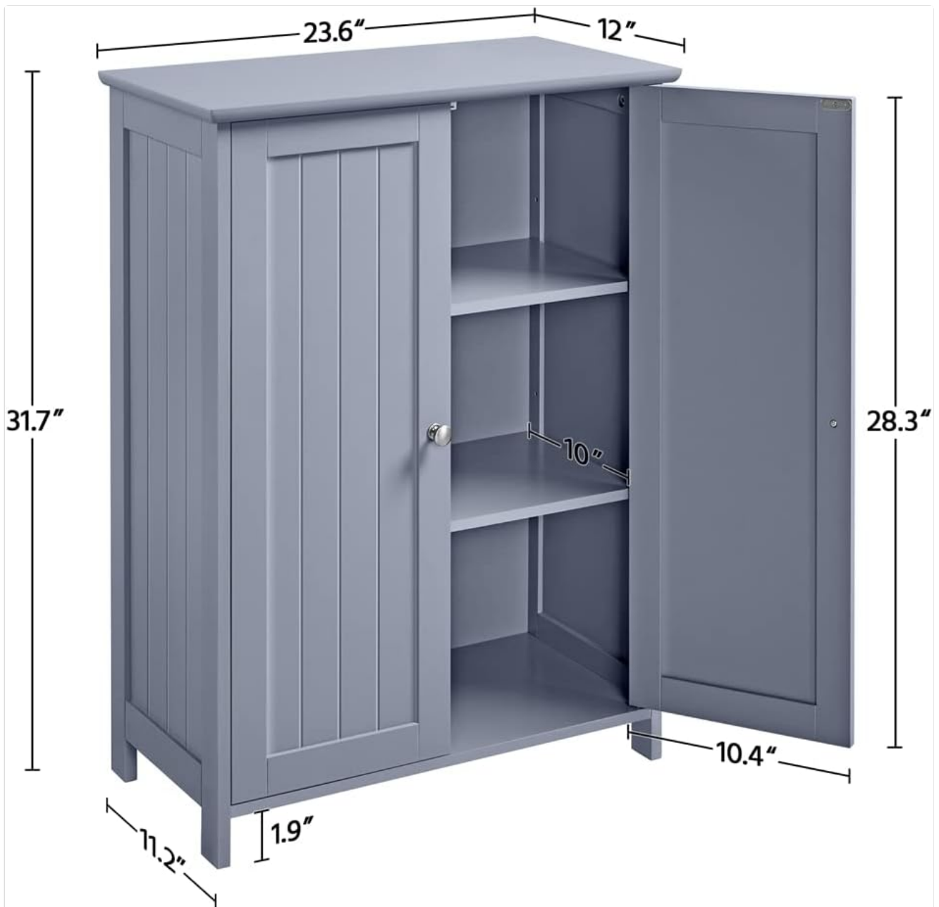
Figure 2.2: Detailed dimensions of the cabinet for precise placement.
