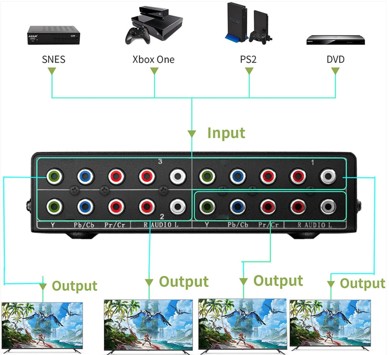
Figure 1: Connection Diagram for BoIAAzUL 1X4 Component Video Audio Splitter. This image illustrates how to connect a single input source (like a PS2 or DVD player) to the splitter's input, and then connect up to four output displays (HDTVs) to the splitter's output ports.
