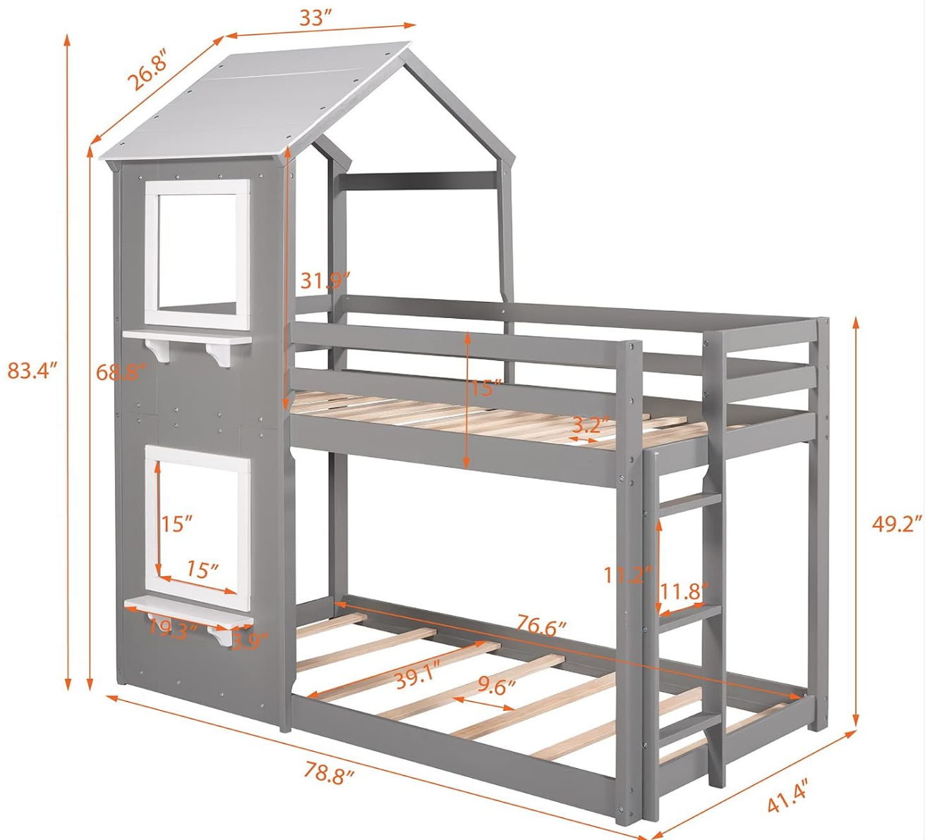
Image 8.1: Dimensional drawing of the SOFTSEA Low Bunk Bed, showing length, width, and height measurements in inches.
