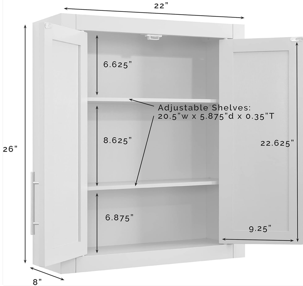
Image: Diagram showing the overall dimensions of the cabinet (22" W x 8" D x 26" H) and internal shelf dimensions.
