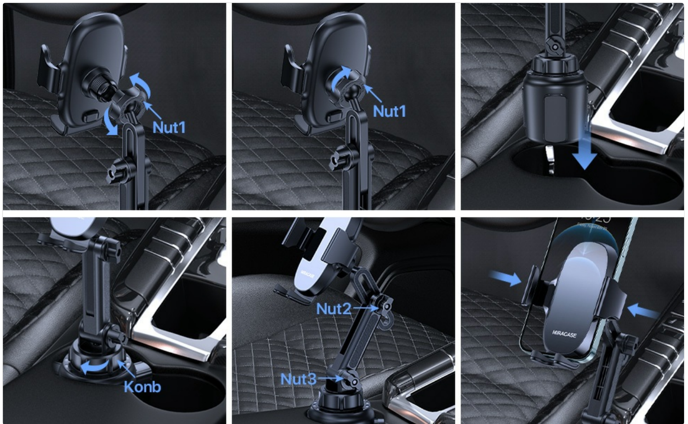
Figure 2: Step-by-step visual guide for assembling and installing the phone holder in a car's cup holder.
