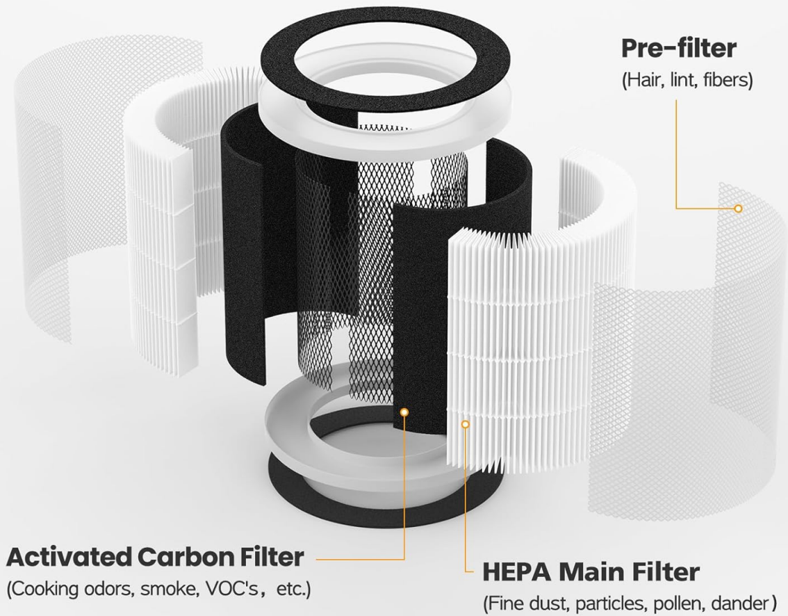
Figure 2: Exploded view of the 3-stage HEPA filtration system, showing the pre-filter, HEPA main filter, and activated carbon filter.
