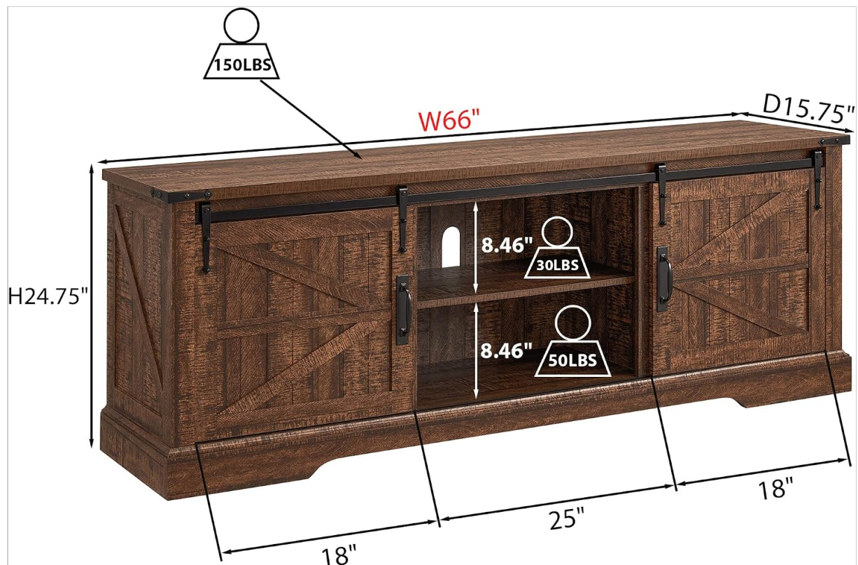
Image 4.1: Dimensional diagram of the TV stand, including weight limits for the top surface (150 lbs) and interior shelves (30 lbs and 50 lbs).
