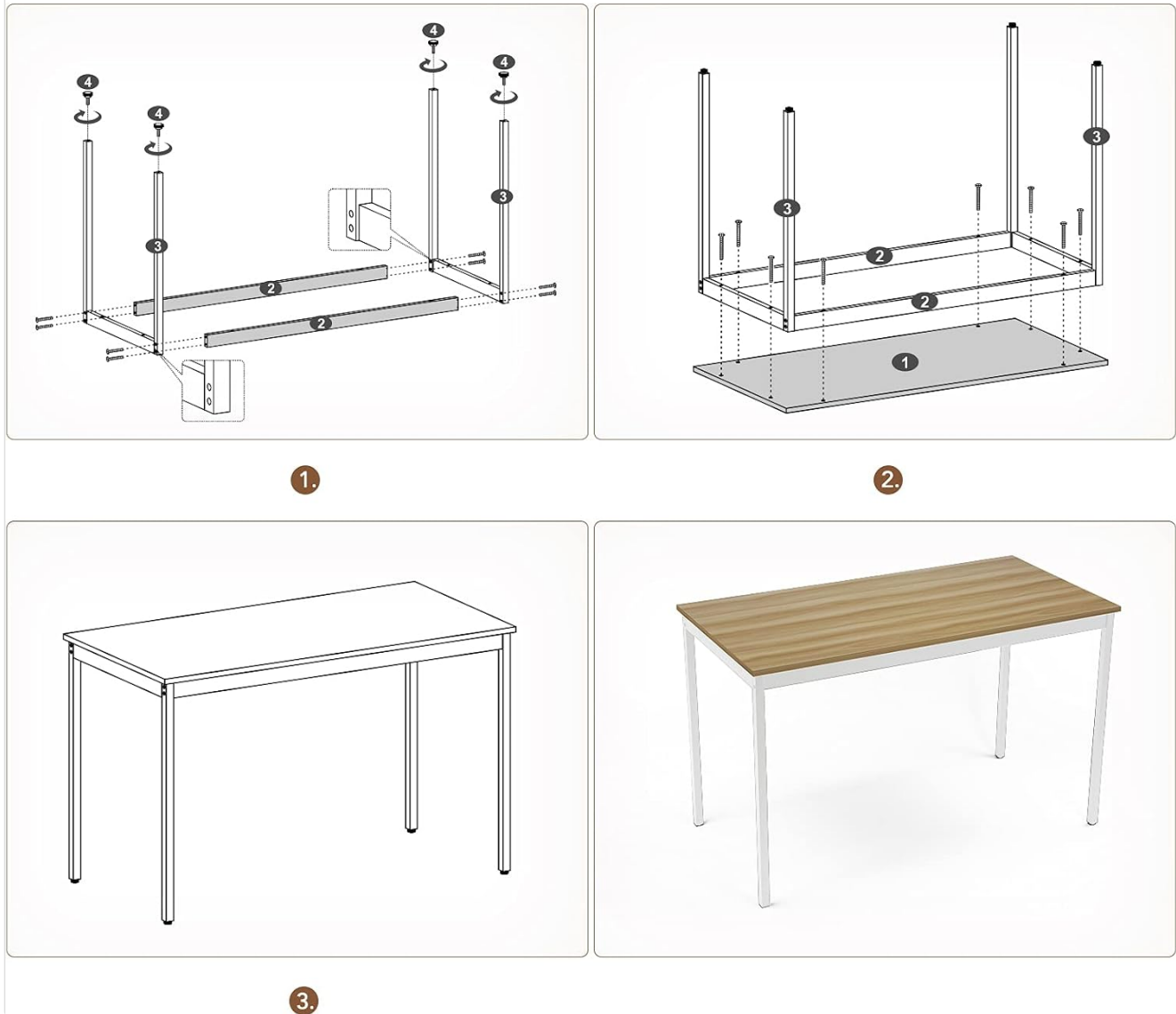
Figure 2: Visual assembly guide.
