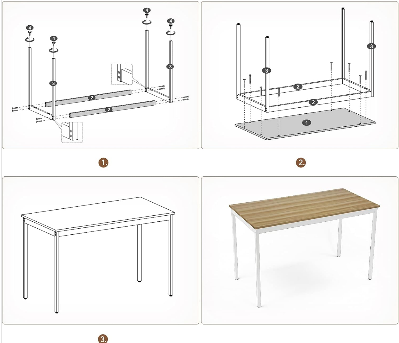
Figure 1: Exploded view of desk components and hardware.
