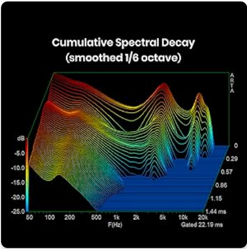
Figure 7: Adjust your audio equalizer settings via the XROUND MyTune App.
