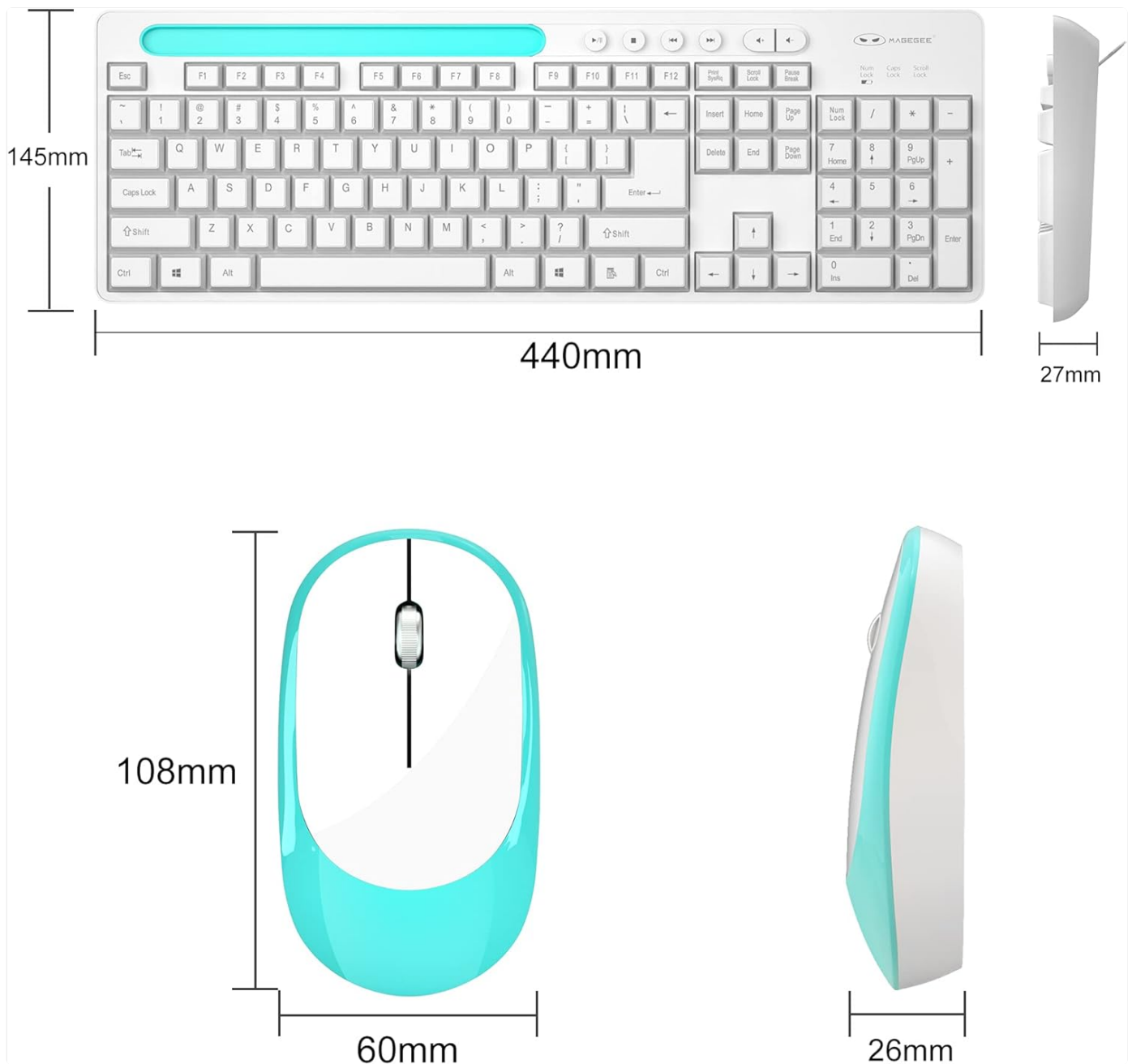
Image: Technical drawing showing the dimensions of the MageGee V620 wireless keyboard: approximately 440mm (length), 145mm (width), and 27mm (height).
