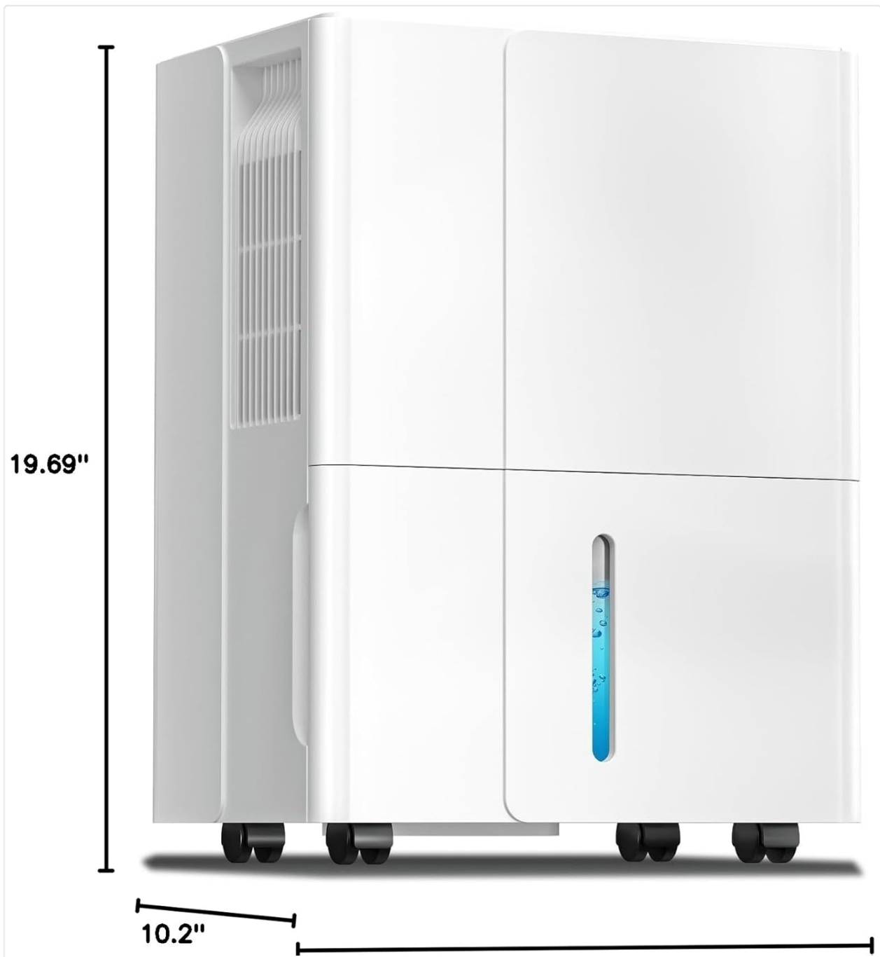
Figure 7.1: Product dimensions for planning placement.
