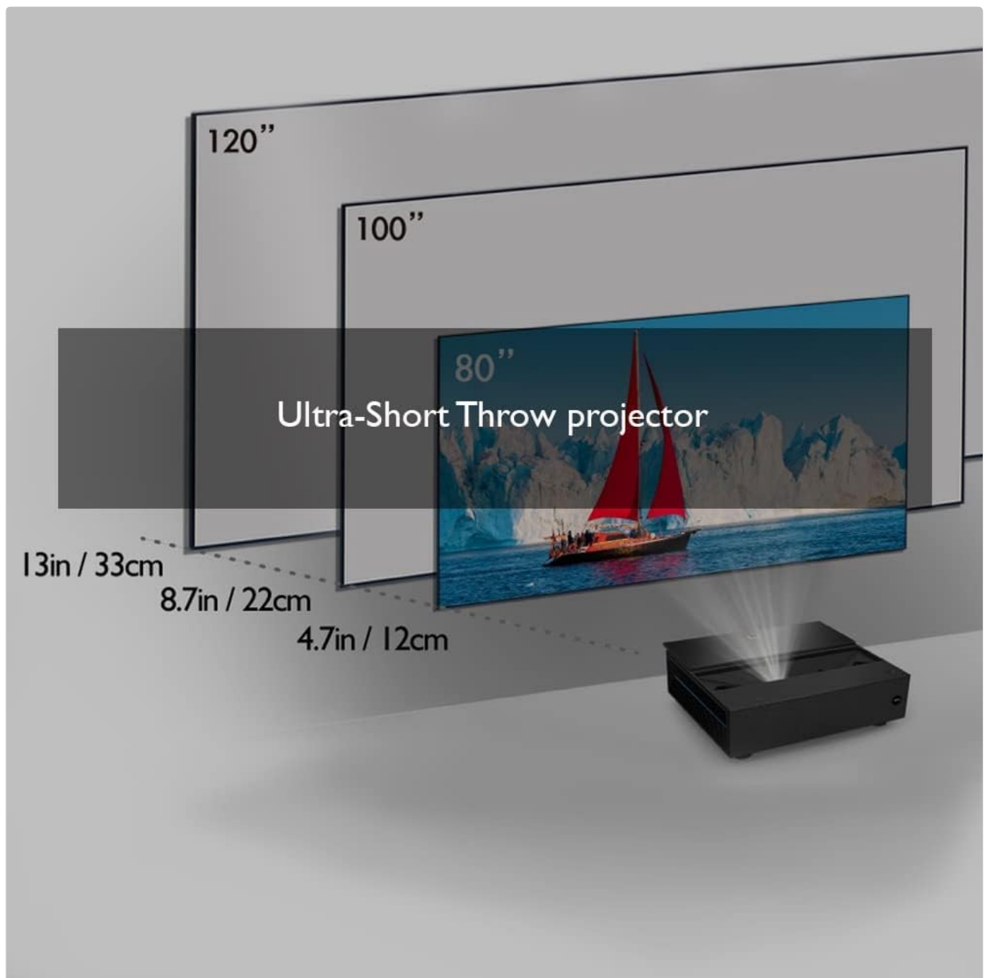
Ultra Short Throw projection distances for various screen sizes.
