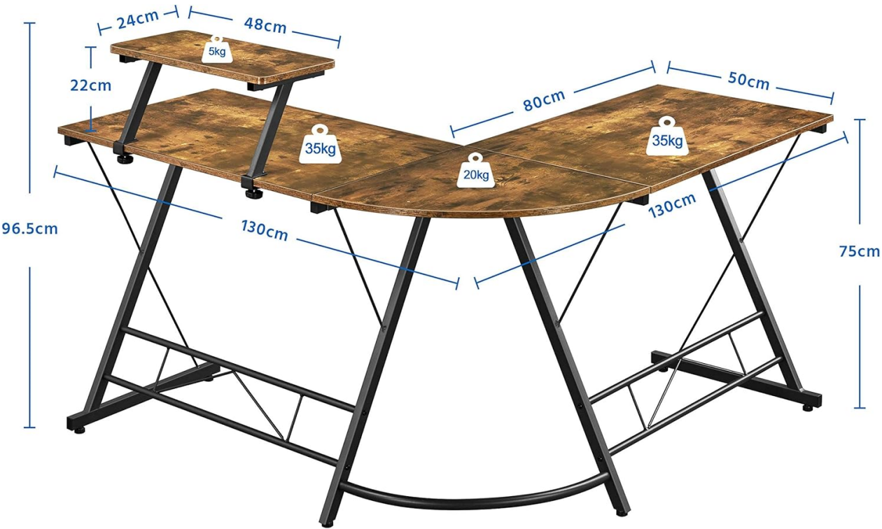
Image: A detailed diagram illustrating the overall dimensions of the L-shaped desk and the monitor stand, including length, width, and height measurements.
