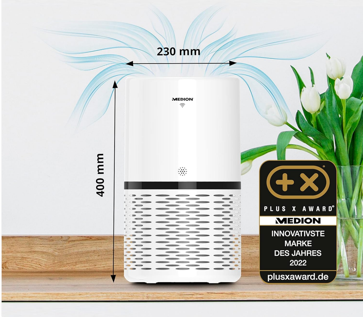
Figure 5: The MEDION MD 10171 Air Purifier shown in a room setting, indicating its suitable room size of 52 m 2 and physical dimensions (400 mm height, 230 mm diameter).
