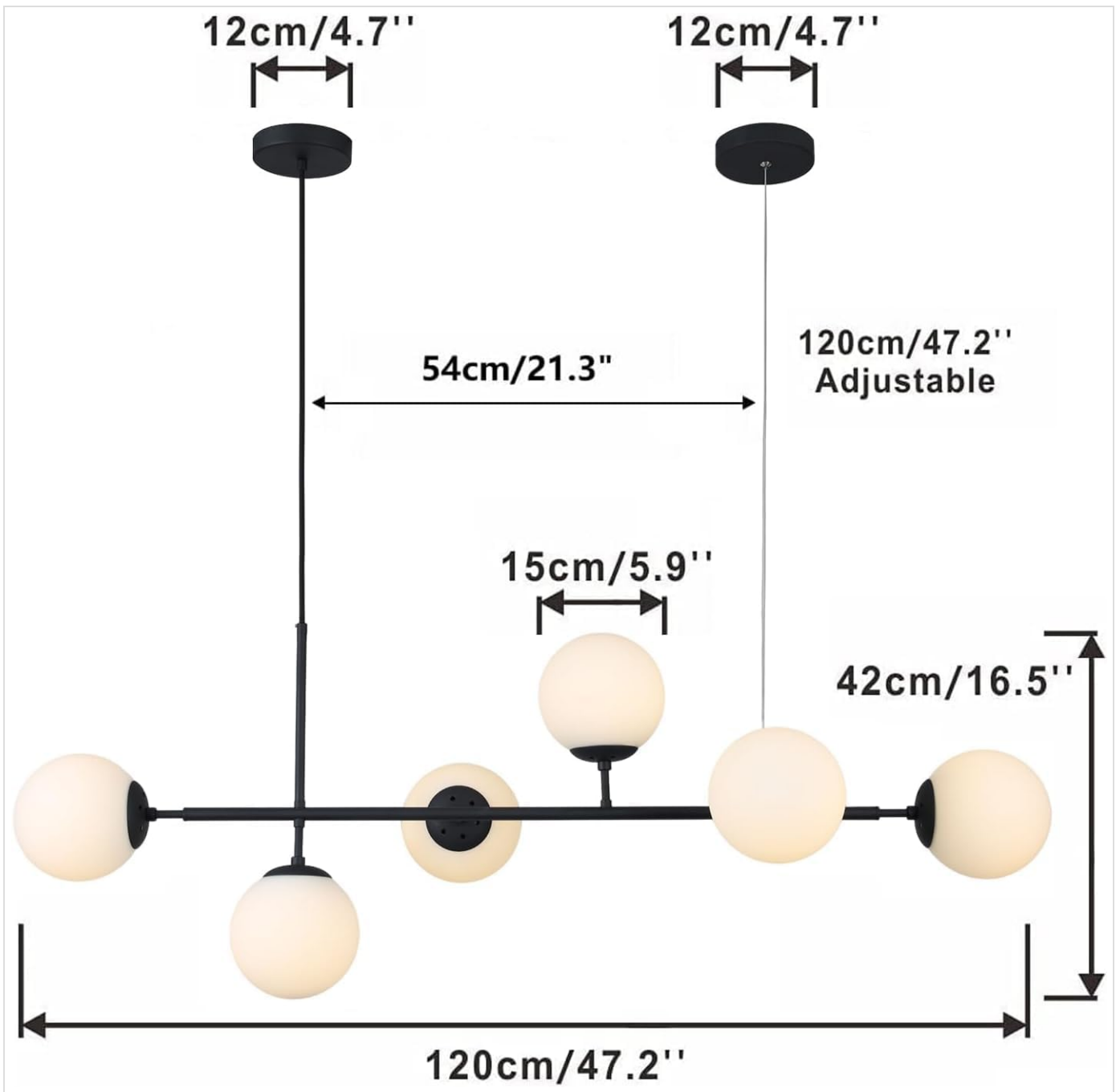
Figure 1: Chandelier Dimensions. Length: 47.2" (120cm), Globe Diameter: 5.9" (15cm), Ceiling Plate: 4.7" (12cm), Adjustable Hanging Cord: 47.2" (120cm).
