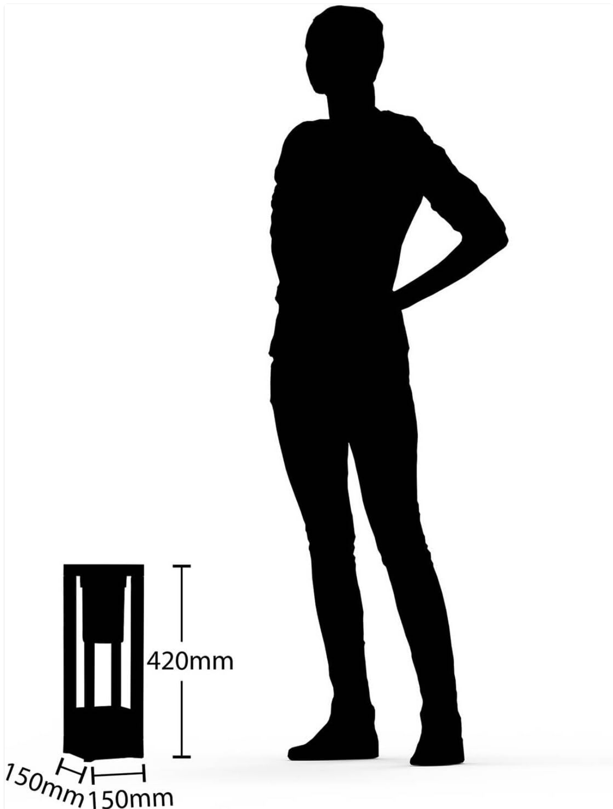
Figure 6: Dimensional drawing of the Lucande Kalisa Pedestal Lamp.
