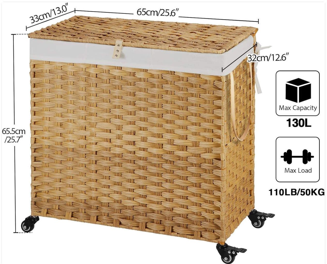
Image: A diagram illustrating the precise dimensions and capacity of the 130L laundry hamper.
