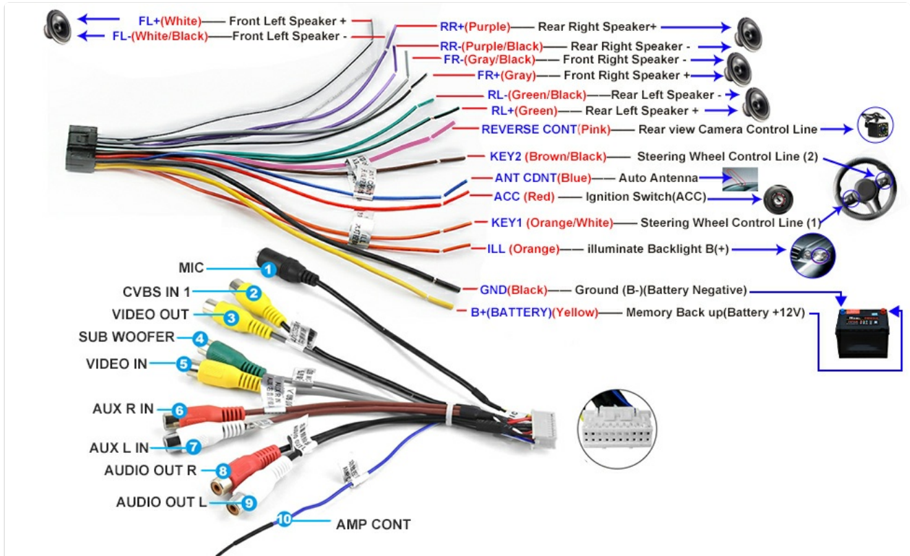
Image: Rear view camera connection diagram.
