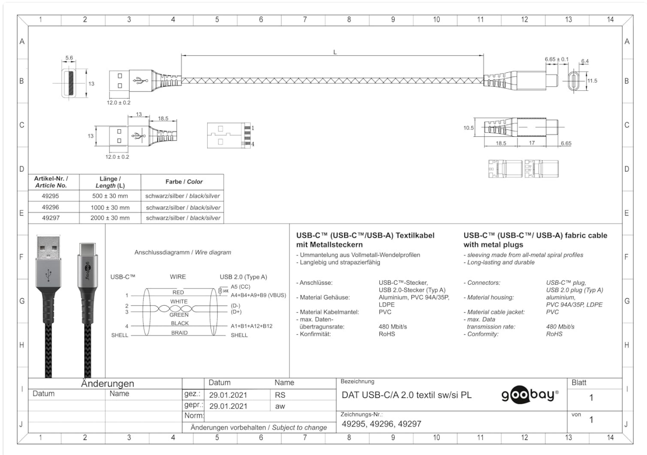
Image 6.1: Detailed technical diagram showing the USB-C and USB-A connectors, dimensions, and internal wiring.
