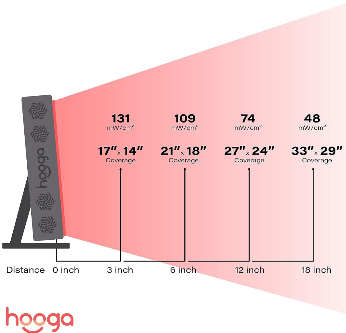
Figure 3: Irradiance and coverage at various distances from the panel.
