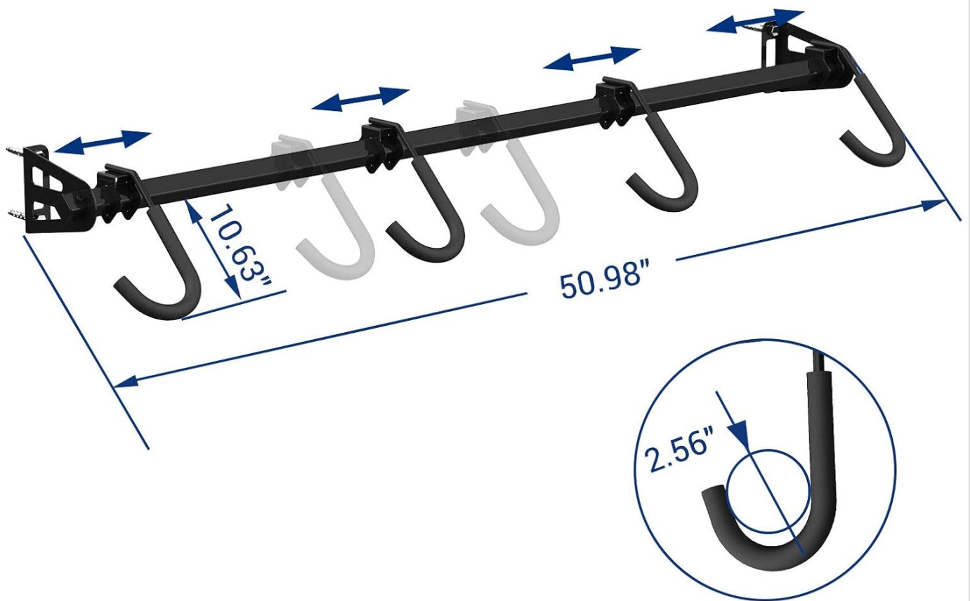
Image: A diagram highlights the adjustable bike hooks, showing how they can be repositioned along the rail to accommodate various bike sizes, along with key dimensions of the rack and hooks.
