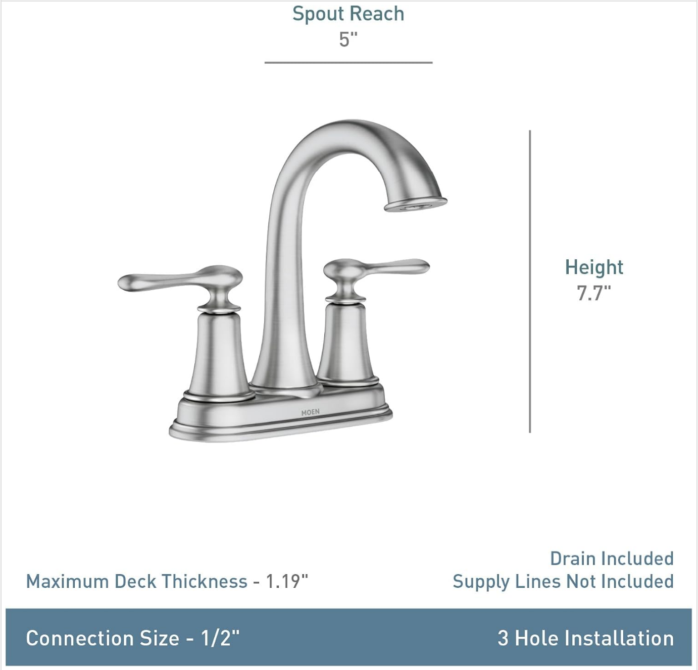
A technical drawing of the Moen Ellicott faucet with key dimensions: spout reach of 5 inches and height of 7.7 inches. It also indicates a maximum deck thickness of 1.19 inches, 1/2 inch connection size, and suitability for 3-hole installation.
