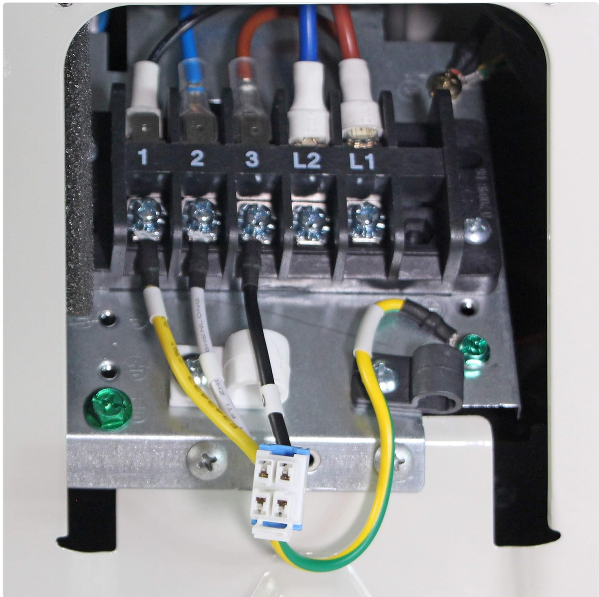
Figure 4: Electrical connections for the outdoor unit.
