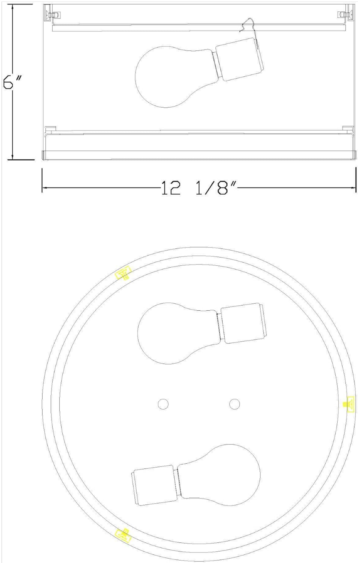
Figure 1: Technical diagram with dimensions (12 1/8" width, 6" height) and internal bulb placement for the Z-Lite 2 Light Flush Mount.
