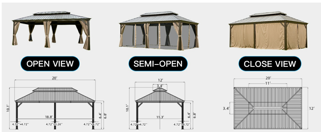
Figure 4: Demonstrates the versatility of the double track system with options for open, semi-open, and closed views.
