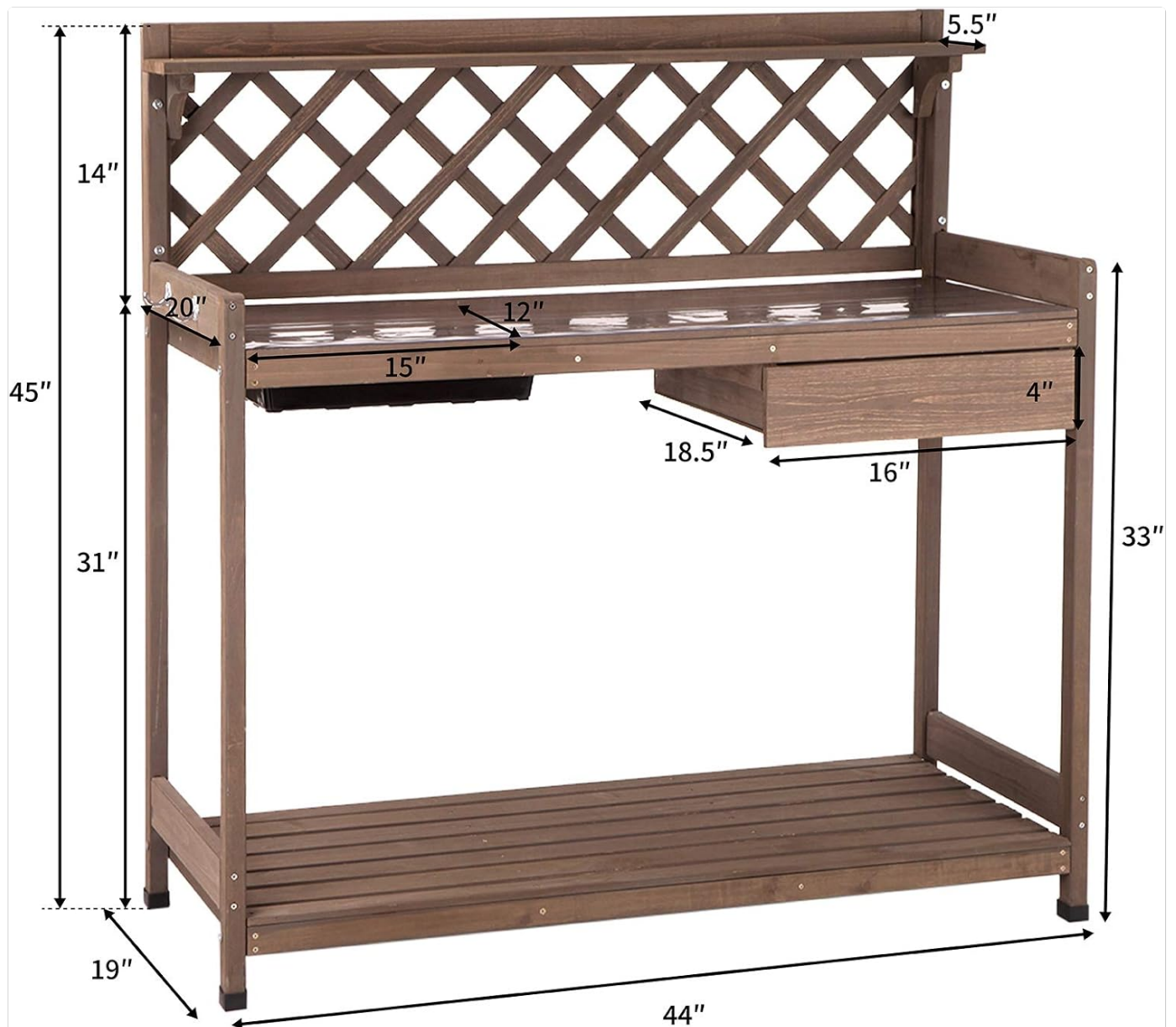
Image: Diagram showing the dimensions of the potting bench, useful for assembly and placement.
