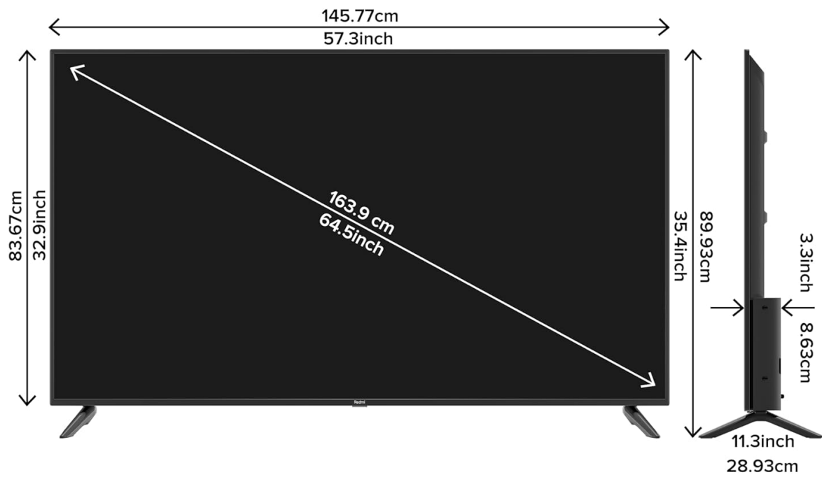
Image: Detailed dimensions of the Redmi 65-inch Smart TV, showing width, height, and depth.
