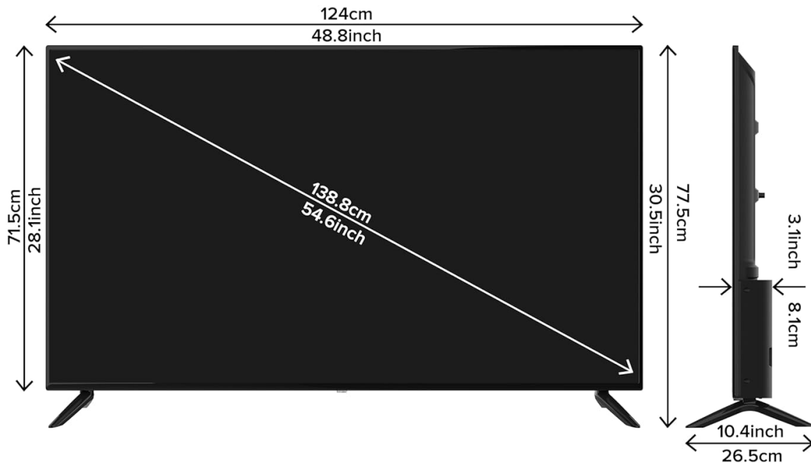
Figure 8: Dimensions of the Redmi Smart TV X55 for planning installation.
