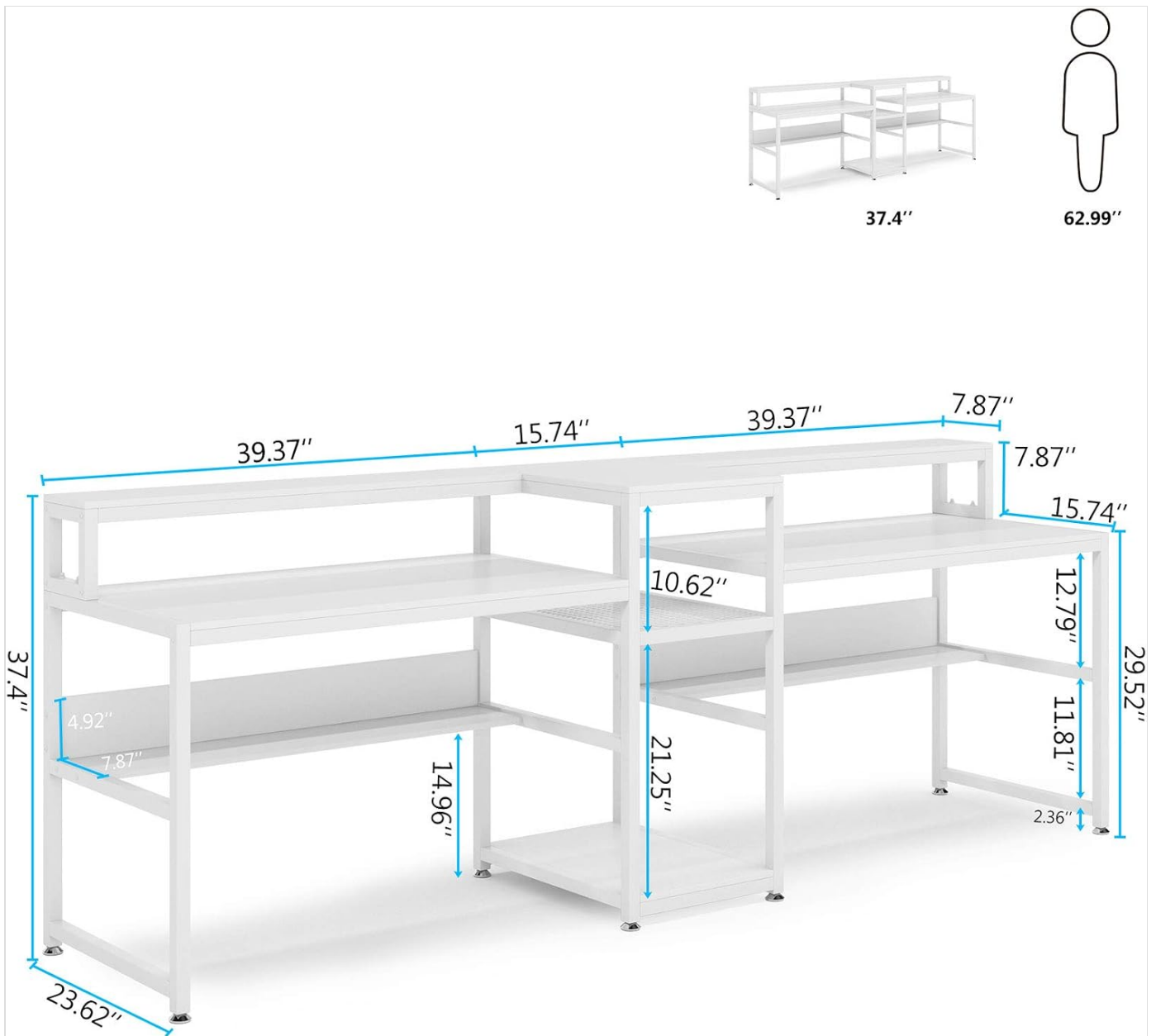
Image: Dimensional diagram of the desk, illustrating key measurements for planning your space.
